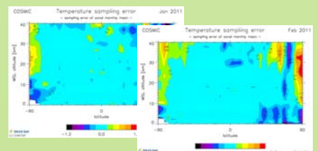
Figure: Estimates of sampling errors in zonal monthly mean temperatures for January and February 2011 based on RO data from the COSMIC mission.
