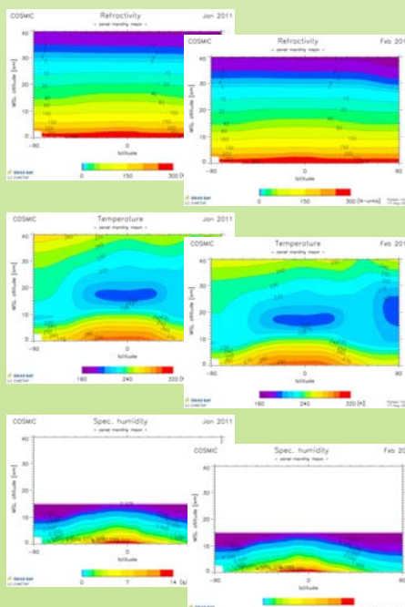
Figure: Example ROM SAF climate data products for January and February 2011 based on FORMOSAT-3/COSMIC data. The data consist of gridded zonal monthly means and related data (standard deviations, error estimates, and estimates of a priori information contents).
